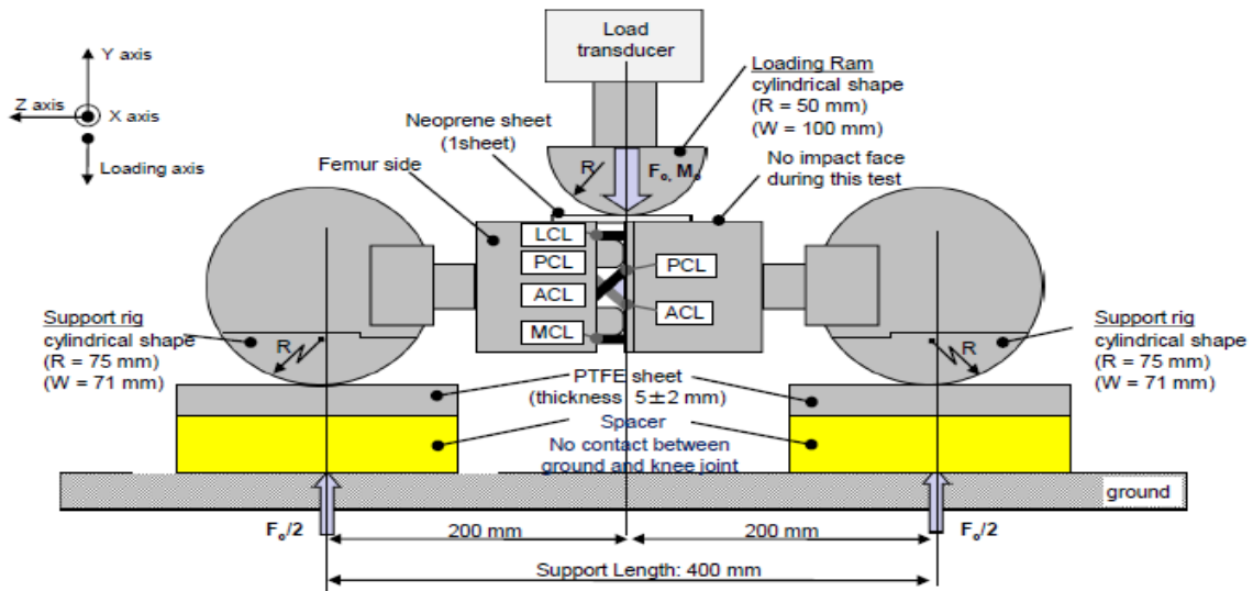
Figure 5 Flexible lower legform impactor: Test set-up for the knee joint in the static certification test (see paragraph 1.2.5. of this annex)
