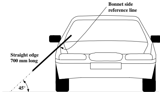
Figure 9 Side reference line
