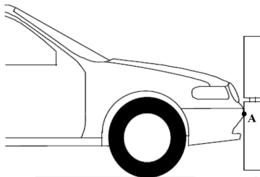
Figure 8B Measuring point in the vertical longitudinal plane through the central axis of the legform impactor (see paragraph 2.28.2.)
