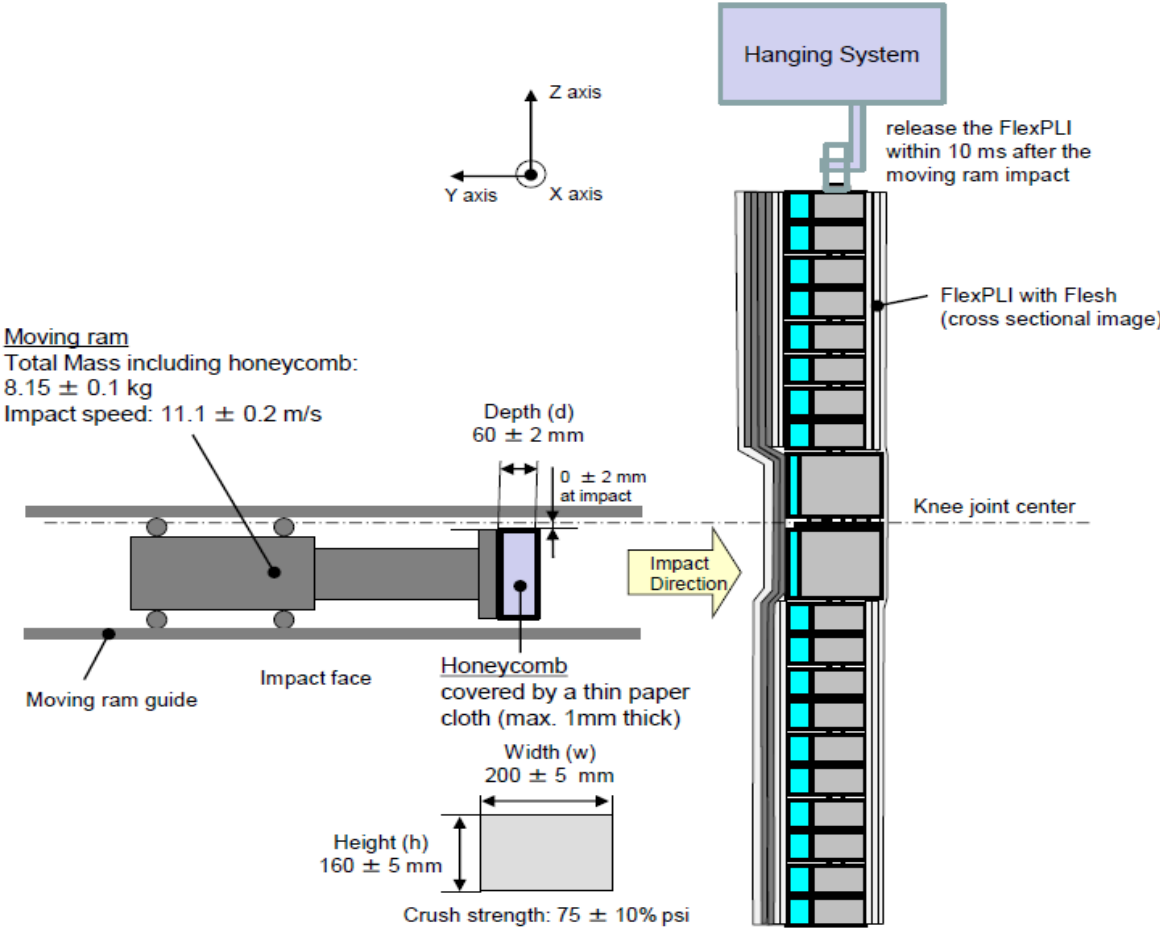
Figure 7 Flexible lower legform impactor: Test set-up for the dynamic lower legform impactor certification test (inverse test, see paragraph 1.4.3.1. of this annex)
