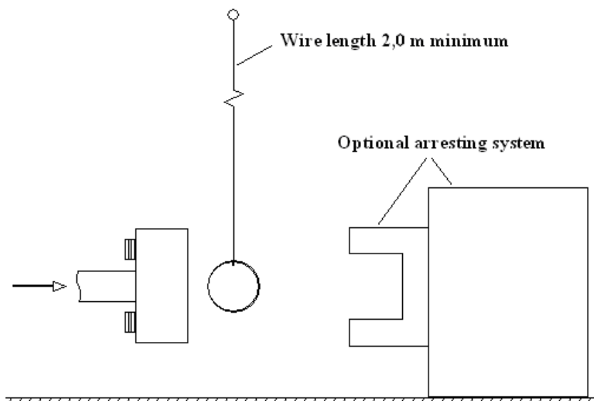
Figure 8 Test set-up for dynamic upper legform impactor certification test
