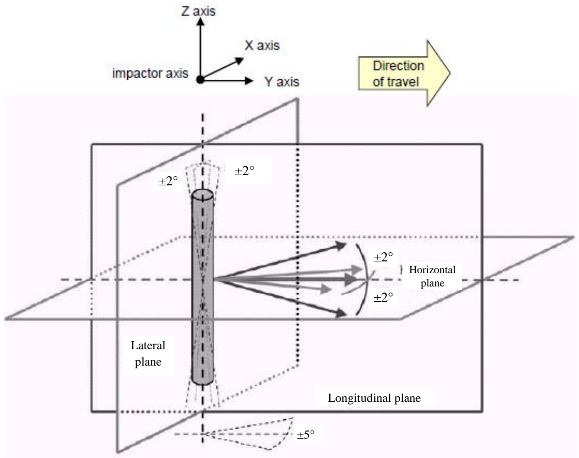
Figure 3 Tolerances of angles for the flexible lower legform impactor at the time of the first impact
