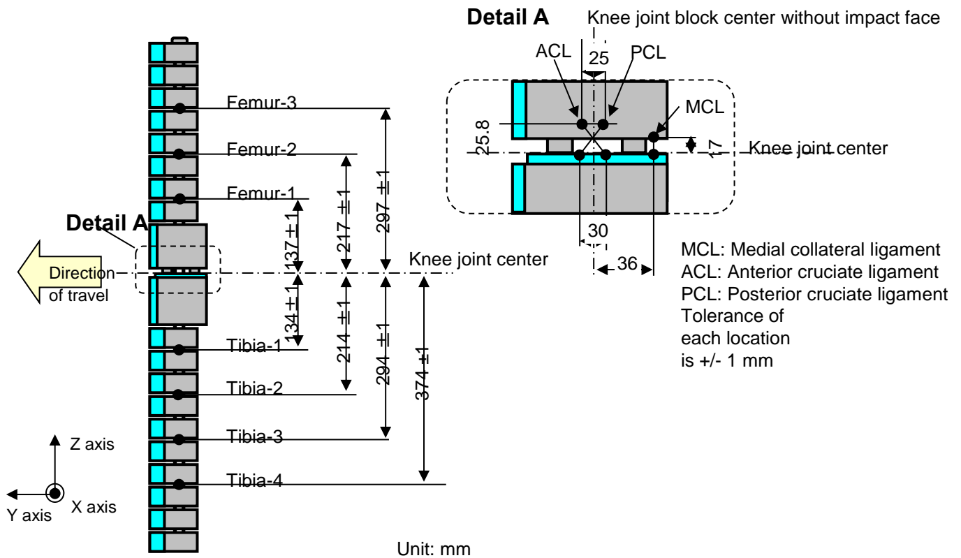
Figure 3 Flexible lower legform impactor instrument locations
