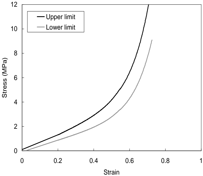
Figure 2 Flexible lower legform impactor: Flesh and skin compression characteristics
