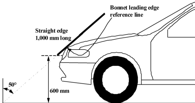
Figure 1 Bonnet leading edge reference line
