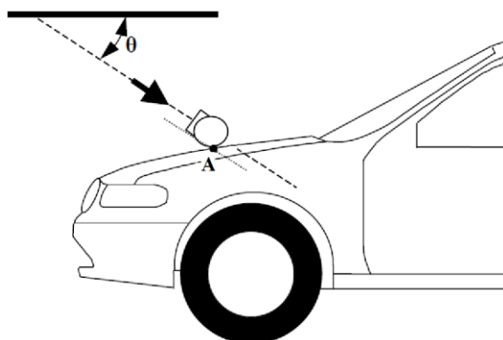
Figure 8A Measuring point in the vertical longitudinal plane through the center of the headform impactor (see paragraph 2.28.1.) 2
