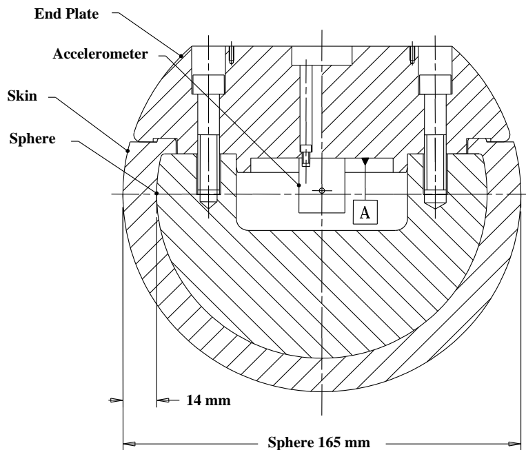
Figure 6 Adult headform impactor
