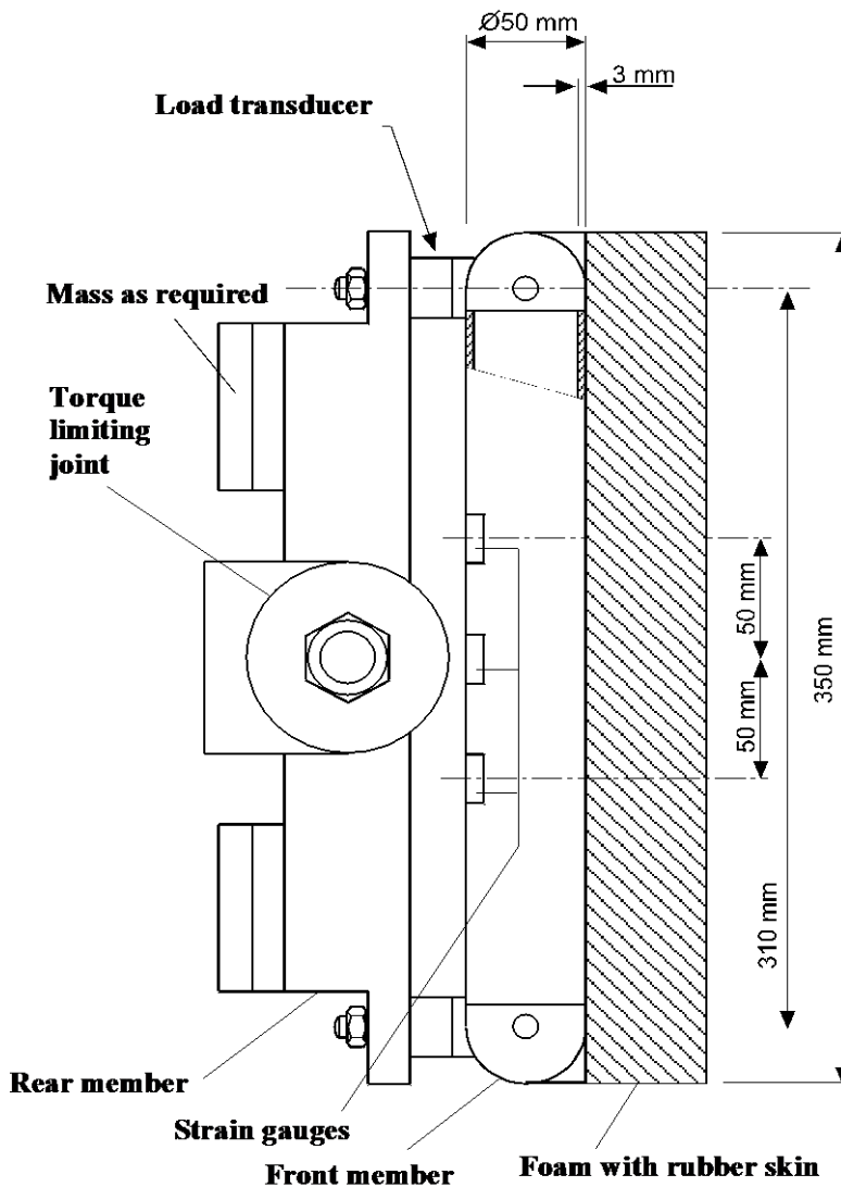
Figure 4 Upper legform impactor
