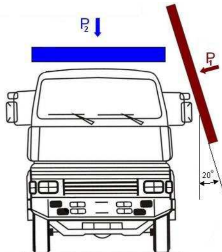
Figure 3 Roof strength test (Test C)
