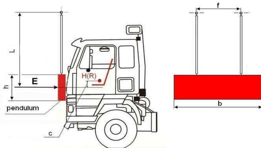
Figure 1 Front impact test (test A)
