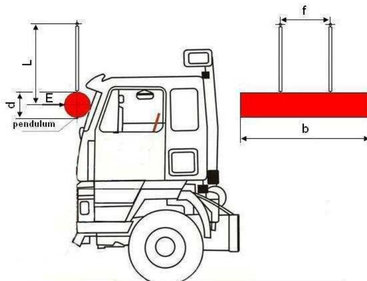
Figure 2 Front pillar impact test (Test B)
