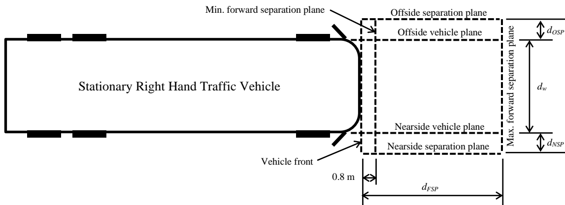
Figure 1 Blind spot boundary test area
