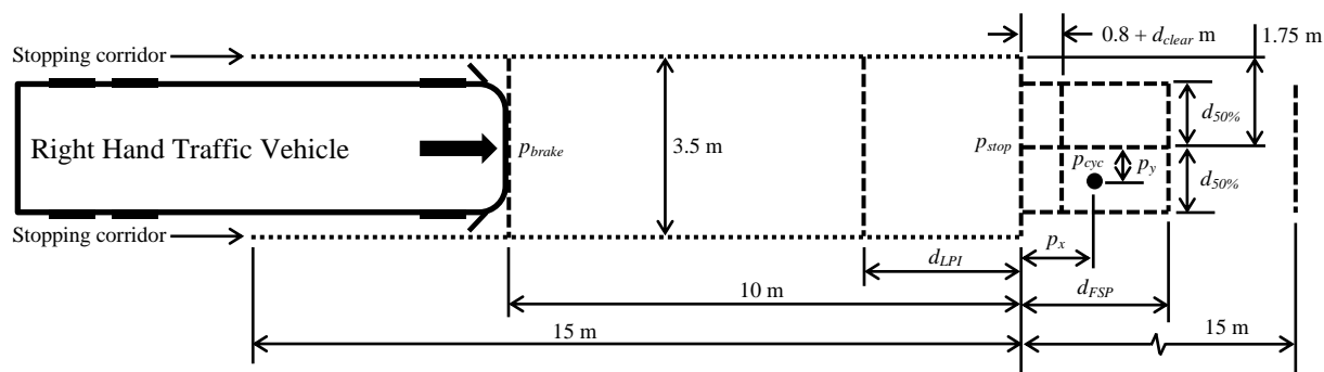
Figure 2 Set Up for Longitudinal Cyclist Tests
